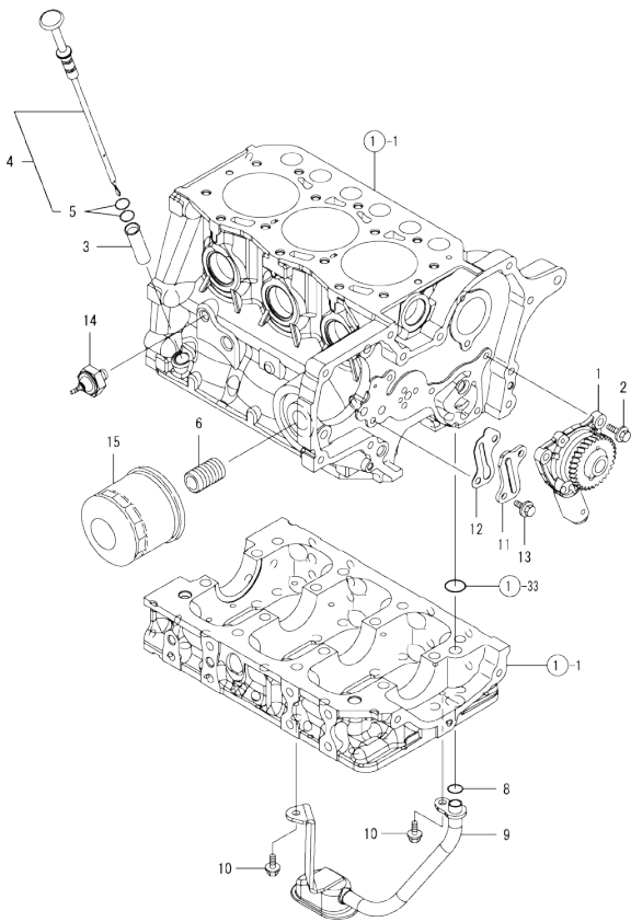
Fig.9. LUB.OIL SYSTEM
