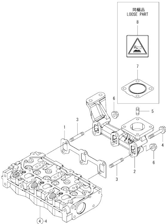
Fig.6. EXHAUST MANIFOLD
